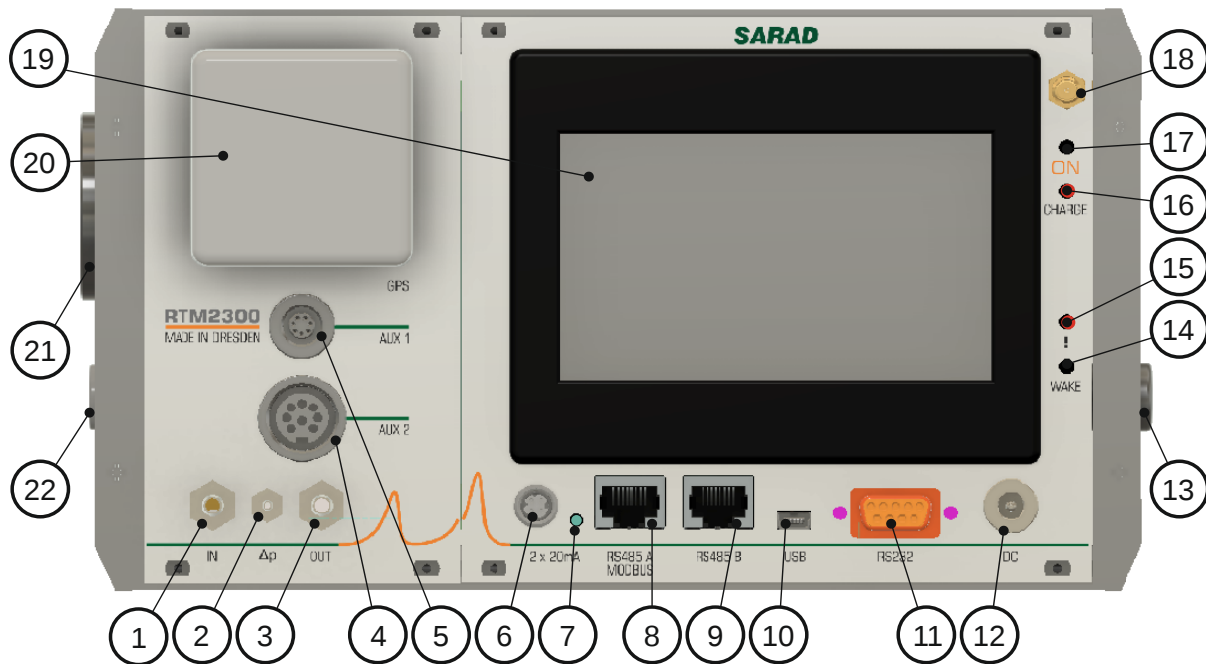
Figure 1 Basic monitor
